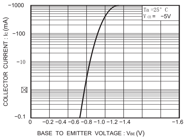
Fig.1 Grounded emitter propagation characteristics
