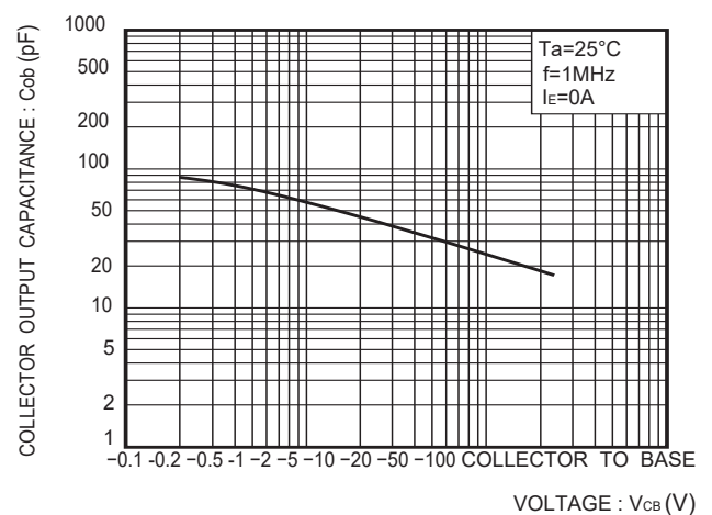
Fig.6 Collector output capacitance vs. collector-base voltage
