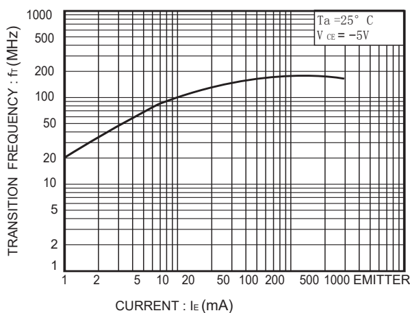
Fig.5 Gain bandwidth product vs. emitter current
